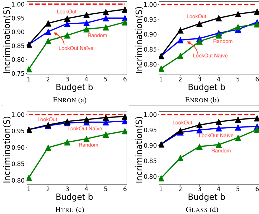
Fig. 4: LOOKOUT explains away top 10-20 outliers with 4-5 plots. Results shown on ENRON (a-b) with k = \{10, 20\} outliers (left to right), HTRU (c) with 32 outliers and GLASS (d) with 28 outliers.
