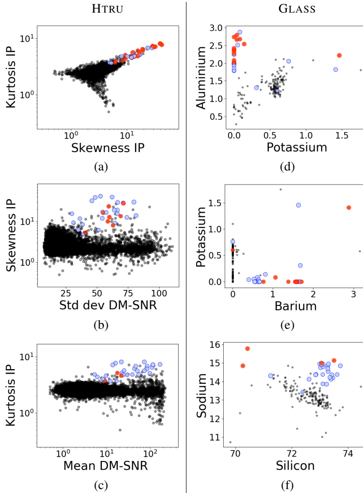
Fig. 7: Discoveries using LOOKOUT on dictated outliers: LOOKOUT explains outlier characteristics on HTRU (a-c) and GLASS (d-f) for budget b = 3 .
